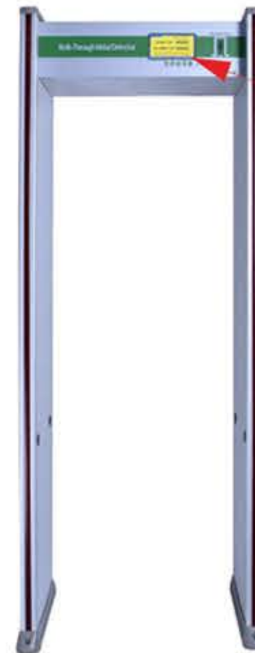
LTAPLCD24 24 Zones, Portable 7 inch LCD Touch Screen,IP65 Optional function: wifi APP for android phone, waterproof cover Part of sensitivity): 255 Whole Security level: 100 Application: 90 places Detect flying objects Frequency: 100(Automatic or Manual) Alarm: 16 kinds of Sound Black/grey shell
